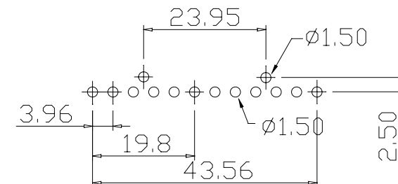
Recommended PCB Layout (PCB TOLERANCE±0.05)
